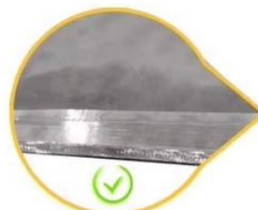
Ours-Edge-mining
