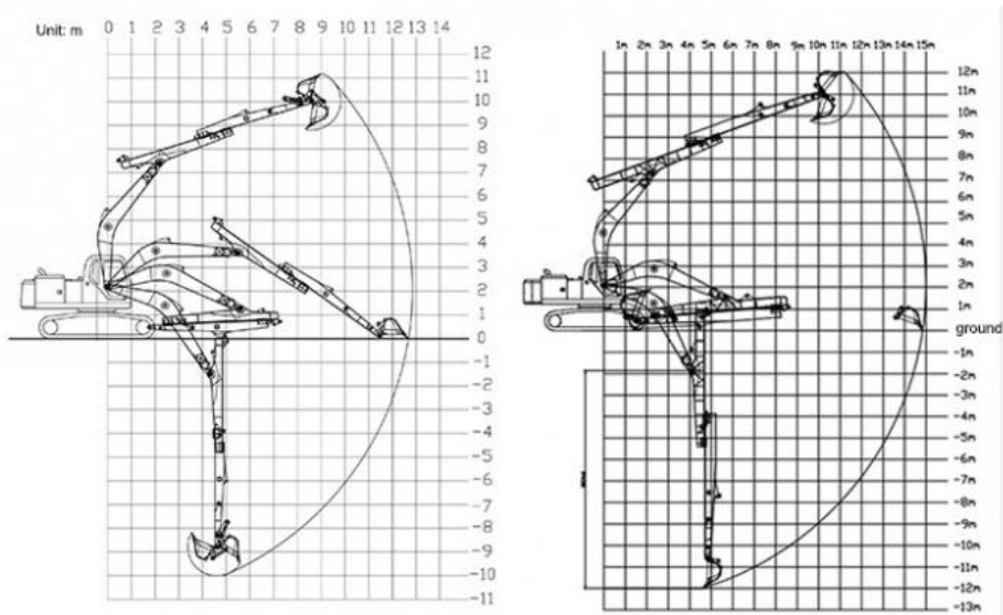
Specifications of one set of telescopic arm for excavator:
